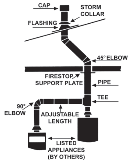
Type BW Gas Vent Multiple Appliance
