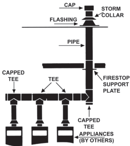
Type BW Gas Vent Multiple Appliance with manifold
